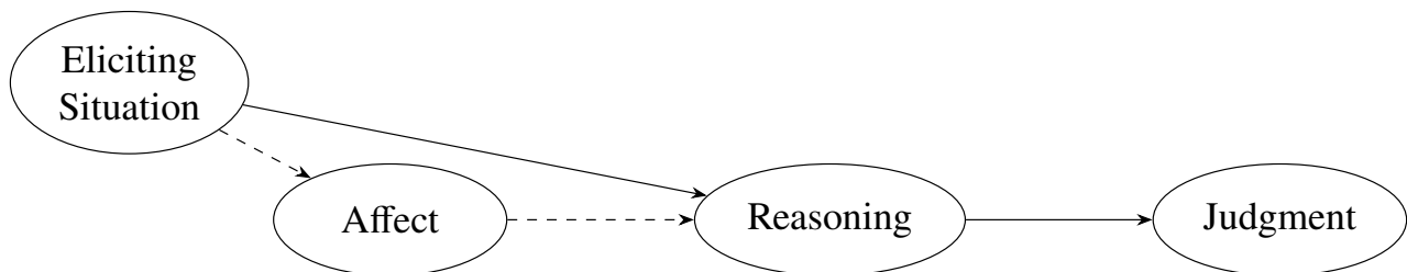
Figure 1: The rationalist model of moral judgment.
