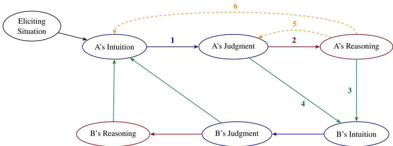
Figure 2: The social intuitionist model of moral judgment.
