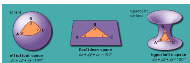
Figure 2: Sum of angles in a triangle
